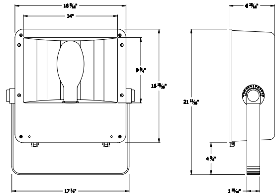
TRUNNION MOUNT
