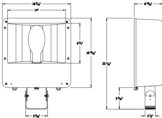
YOKE MOUNT
